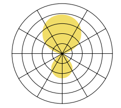
koi-q standing light/ desk mounted luminaire 114lm/W@4000K
