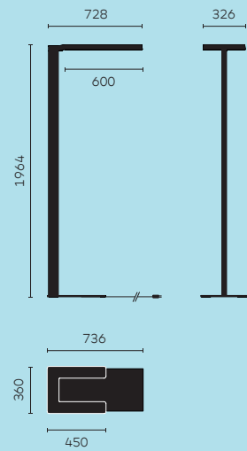
bob floor light
